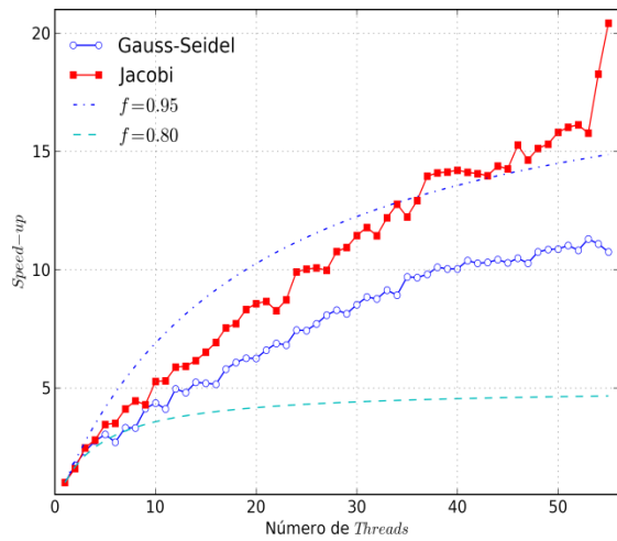
d) Speed-up para N = 4097 \times 4097
