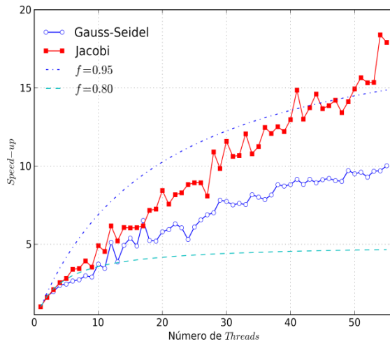
c) Speed-up para N = 2049 \times 2049
