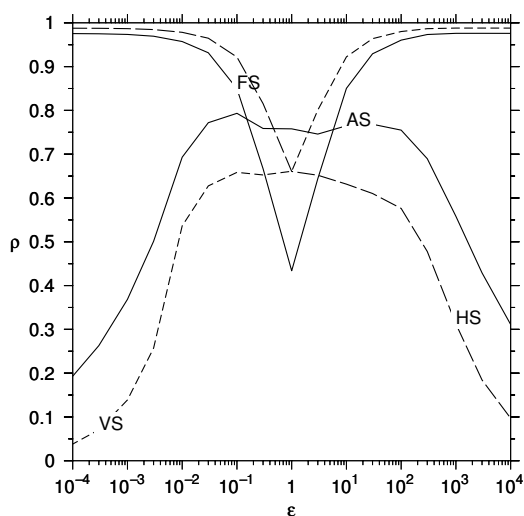
Figure 3.15: Numerically observed convergence factors “per work unit” for multigrid waveform relaxation with different smoothers and standard coarsening, applied to the anisotropic diffusion equation. ( \beta = 0 , h = 2^{-5} , \Delta t = 10^{-3} , BDF1, V-cycle )
