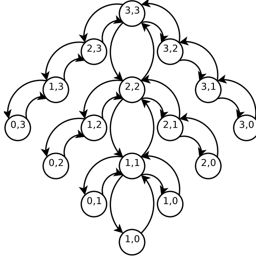
Figure 3.7: MGS iteration using V-cycles for standard coarsening, x -semicoarsening presmoothing and y -semicoarsening postsmoothing.
