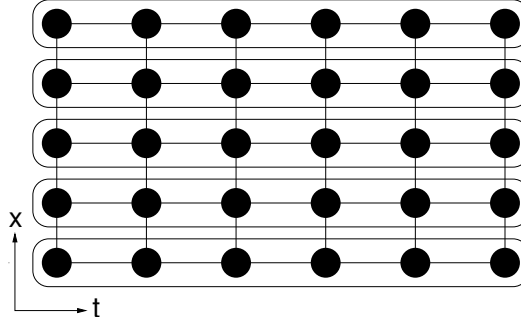
Figure 4.5: In a waveform relaxation procedure all the values for one spatial grid point are updated simultaneously.
