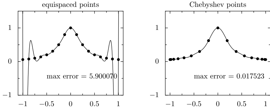
Figure 5.1: The function (1+16x^2)^{-1} interpolated by polynomials of degree 16 on equidistant and Chebyshev meshes.
