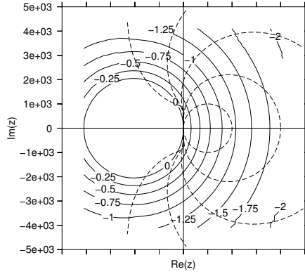
Figure 3.12: Spectral picture for two-grid waveform relaxation with red-black Gauss-Seidel as smoother and standard coarsening, applied to the discretized anisotropic diffusion equation. ( \varepsilon = 10^{-3} , \beta = 0 , h = 2^{-5} ) The solid lines represent contour lines of \log_{10}(\rho(M(z))) , the dashed lines represent the scaled boundary loci of BDF1 to BDF5 ( \Delta t = 10^{-3} ).
