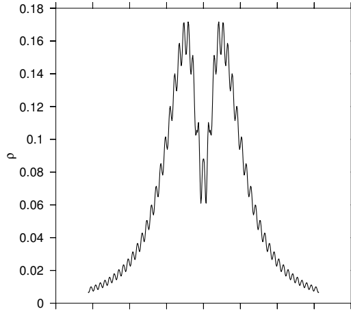
Figure 6.3: \rho(M(i\xi)) for d = 10 , a = 1 , b = -1 , \tau = 1 .
