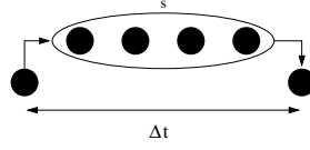
Figure 4.2: An implicit Runge-Kutta method uses intermediate values to advance one time step.
