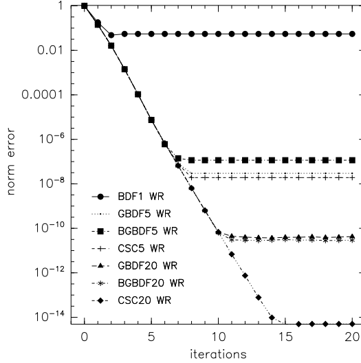
Figure 5.7: Error convergence.
