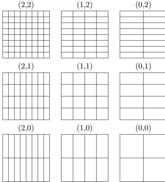
Figure 3.6: A hierarchy of grids for multigrid methods solving a PDE, discretized on grid (2, 2) . Standard coarsening uses the grids (2, 2) , (1, 1) , (0, 0) . Semicoarsening in the x -direction uses the grids (2, 2) , (1, 2) , (0, 2) .
