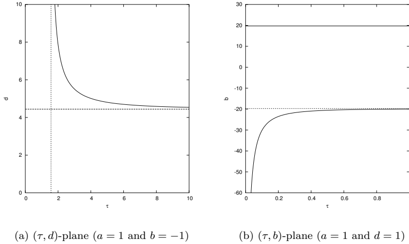
Figure 6.1: Stability regions for the model problem.
