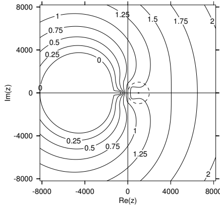
Figure 2.4: Contour lines of the convergence rate R(M(z)) based on a two-grid Fourier mode analysis. The boundary of the scaled stability domain for the implicit Euler method with \Delta t = 1/1024 is also shown (dashed line).
