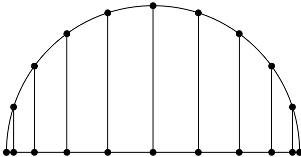
Figure 5.2: The Gauss-Chebyshev-Lobatto points.
