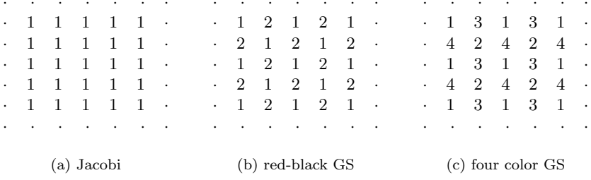
Figure 3.2: Grid points that can be updated simultaneously for Jacobi, red-black and four color Gauss-Seidel relaxation.
