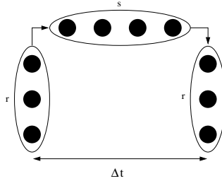
Figure 4.3: A general linear method method uses intermediate values to update several values.
