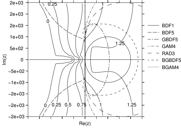
Figure 4.7: Contour lines of the convergence rate R(z) = -\log_{10} \rho(M(z)) and boundaries of the sets \Sigma for discrete waveform relaxation on infinite time domains. The boundary for the BGAM4 discretization coincides with the imaginary axis.
