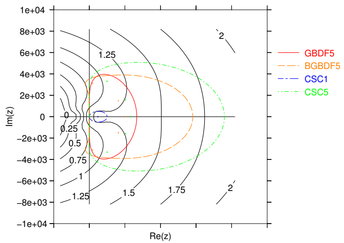
Figure 5.6: Spectral picture.
