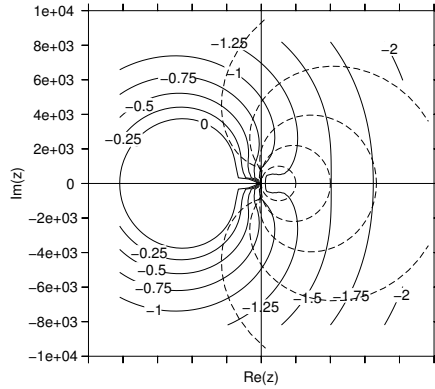
Figure 3.11: Spectral picture for two-grid waveform relaxation with red-black Gauss-Seidel as smoother and standard coarsening, applied to the discretized isotropic diffusion equation ( \varepsilon = 1 , \beta = 0 , h = 2^{-5} ). The solid lines represent contour lines of \log_{10}(\rho(M(z))) , the dashed lines represent the scaled boundary loci of the BDF1-5 methods ( \Delta t = 10^{-3} ).
