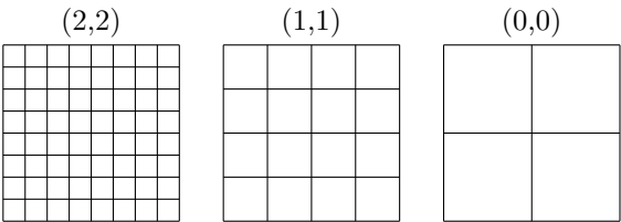
Figure 3.4: A standard coarsening grid hierarchy for multigrid methods solving a PDE, discretized on grid (2, 2) .
