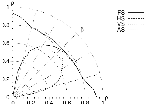
Figure 3.14: Polar plot (\rho, \beta) of numerically observed convergence factors for multigrid waveform relaxation with different smoothers and standard coarsening, applied to the rotated anisotropic diffusion equation. ( \varepsilon = 10^{-3} , h = 2^{-5} , \Delta t = 10^{-3} , BDF1, V-cycle )
