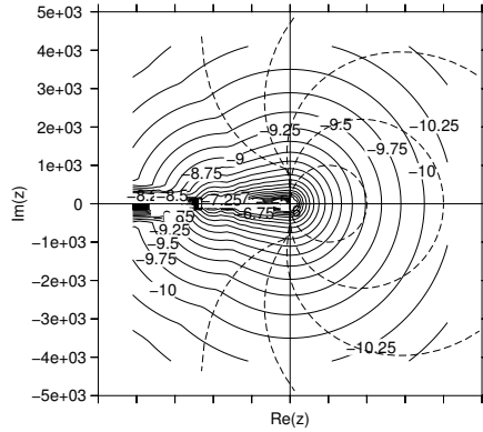
Figure 3.13: Spectral picture for two-grid waveform relaxation with vertical zebra Gauss-Seidel as smoother and standard coarsening, applied to the discretized anisotropic diffusion equation. ( \varepsilon = 10^{-3} , \beta = 0 , h = 2^{-5} ) The solid lines represent contour lines of \log_{10}(\rho(M(z))) , the dashed lines represent the scaled boundary loci of BDF1 to BDF5 ( \Delta t = 10^{-3} ).
