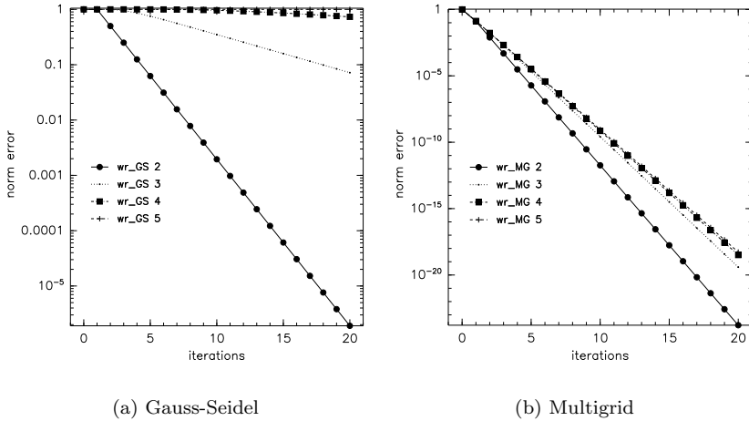
Figure 2.7: Reduction of the error for a Gauss-Seidel and a multigrid wave-form relaxation applied to the discretized heat equation for n_x = n_y = 2^{l+1} , l = 2, \dots, 5 , n_t = 1024 , \Delta t = 1 .
