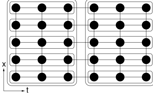
Figure 4.6: Block time stepping can be seen as intermediate between time stepping and waveform relaxation.
