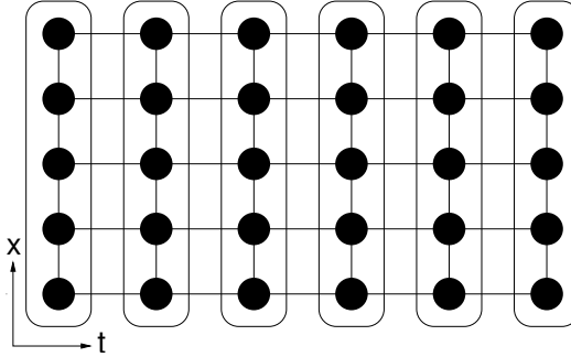
Figure 4.4: In a time stepping procedure all the values for one time step are updated simultaneously.
