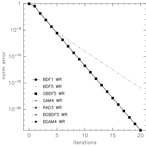
Figure 4.8: Convergence of MGS method (diffusion equation with varying coefficients).
