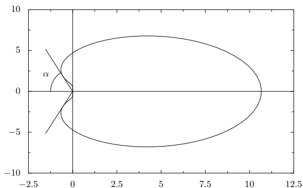
Figure 5.5: Boundary of the stability domain and corresponding sector S_\alpha for the BDF method of order 3 ( \alpha = 73^\circ ).
