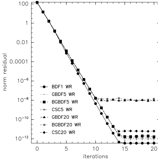
Figure 5.8: Residual convergence.
