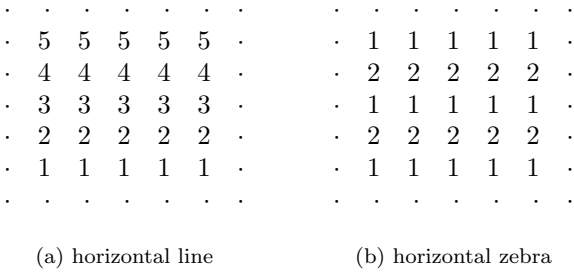
Figure 3.3: Grid points that can be updated simultaneously for horizontal line and zebra relaxation.
