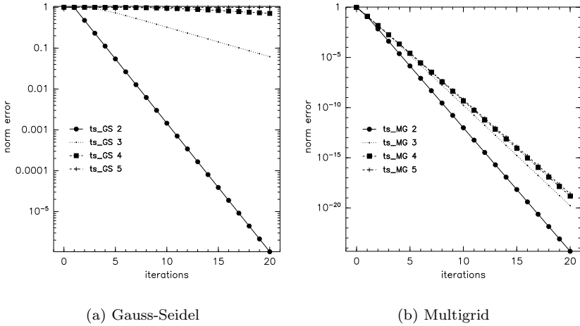
Figure 2.6: Reduction of the error for a Gauss-Seidel and a multigrid method applied to the discretized heat equation for n_x = n_y = 2^{l+1} , l = 2, \dots, 5 , n_t = 1 , \Delta t = 1 .
