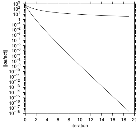
Figure 3.10: Norm of defect for single-grid waveform relaxation (upper curve, red-black Gauss-Seidel) and multigrid waveform relaxation (lower curve, red-black Gauss-Seidel smoother, full-weighting restriction, bilinear interpolation, V(1,1)-cycle). ( \varepsilon = 1 , \beta = 0 , h = 2^{-5} , \Delta t = 10^{-3} , T = 1 )
