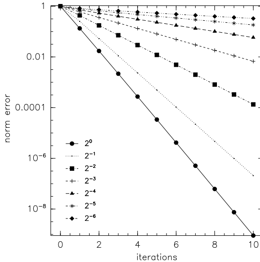
Figure 3.1: Convergence of standard multigrid for stationary anisotropic diffusion equation for various values of \varepsilon .
