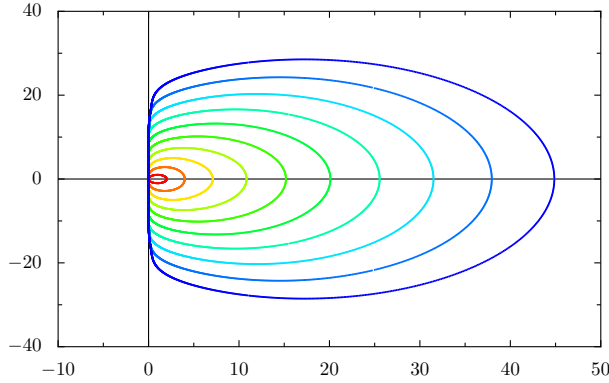
Figure 5.3: Stability domain boundaries for the Chebyshev spectral collocation methods of orders 1 to 10.
