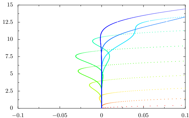
Figure 5.4: Detail of Figure 5.3 near the imaginary axis.
