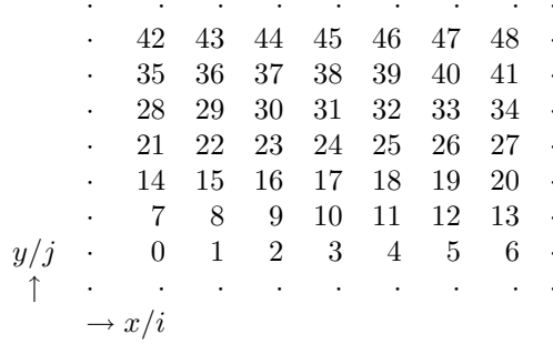
Figure 2.1: Lexicographical ordering for a rectangular grid ( n_x = n_y = 8 ).
