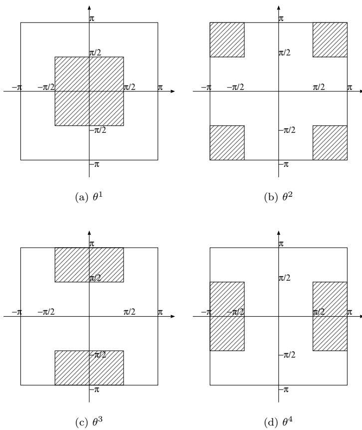
Figure 3.8: Wavenumbers of related exponential Fourier modes.
