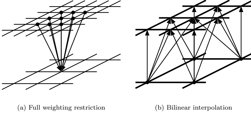
Figure 3.5: Schematic representation of the intergrid operators.
