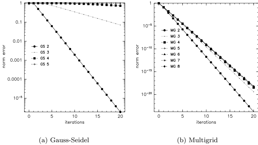
Figure 2.5: Reduction of the error for a Gauss-Seidel and a multigrid method applied to the discretized Poisson equation for n_x = n_y = 2^{l+1} , l = 2, 3, \dots
