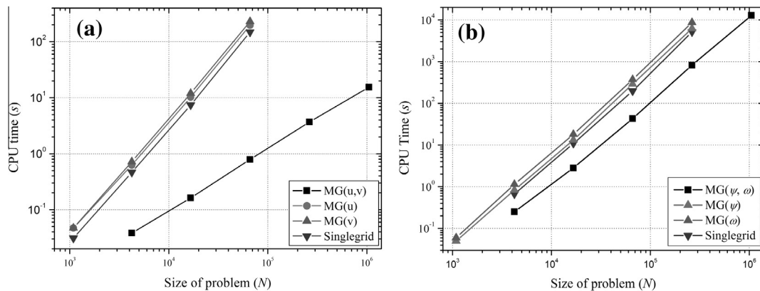
Fig. 9. Performance of the multigrid method when applied to only one equation in problems with two equations: (a) Burgers equations; (b) Navier–Stokes equations in streamfunction–vorticity formulation.
