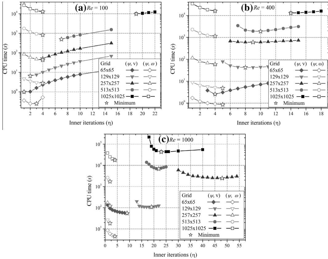
Fig. 4. Effect of the number of inner iterations ( \eta ) on the CPU time for the Navier–Stokes equations in two formulations for different grids.
