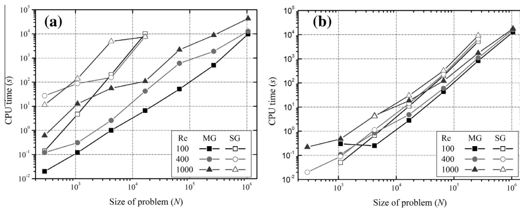
Fig. 8. Multigrid vs. singlegrid performance for both formulations: (a) streamfunction–velocity formulation; (b) streamfunction–vorticity formulation.
