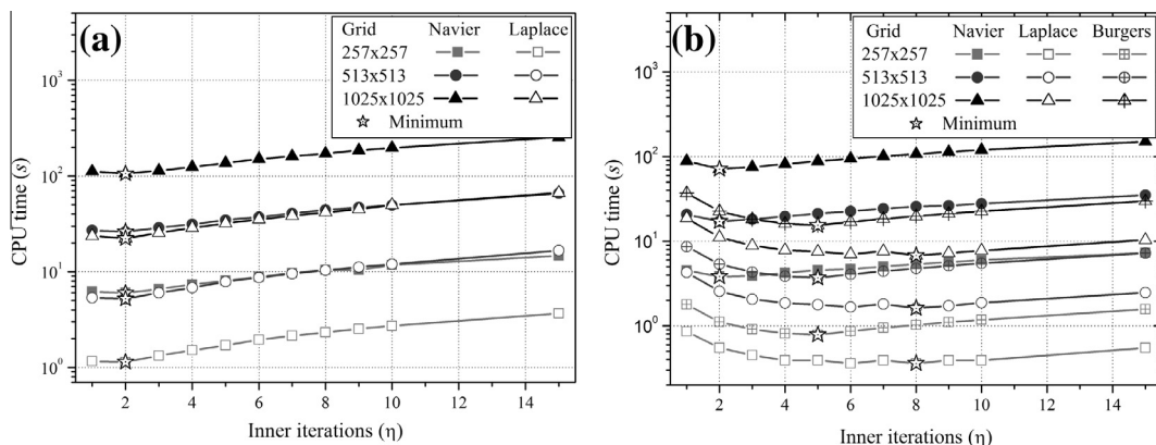
Fig. 3. Effect of the number of inner iterations ( \eta ) on the CPU time in different grids: (a) CS scheme; (b) FAS scheme.
