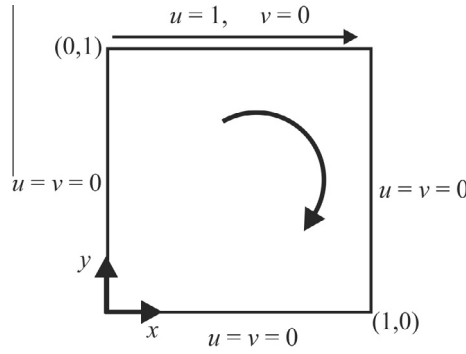
Fig. 2. Boundary conditions of the velocities in lid-driven cavity for the Navier–Stokes equations.
