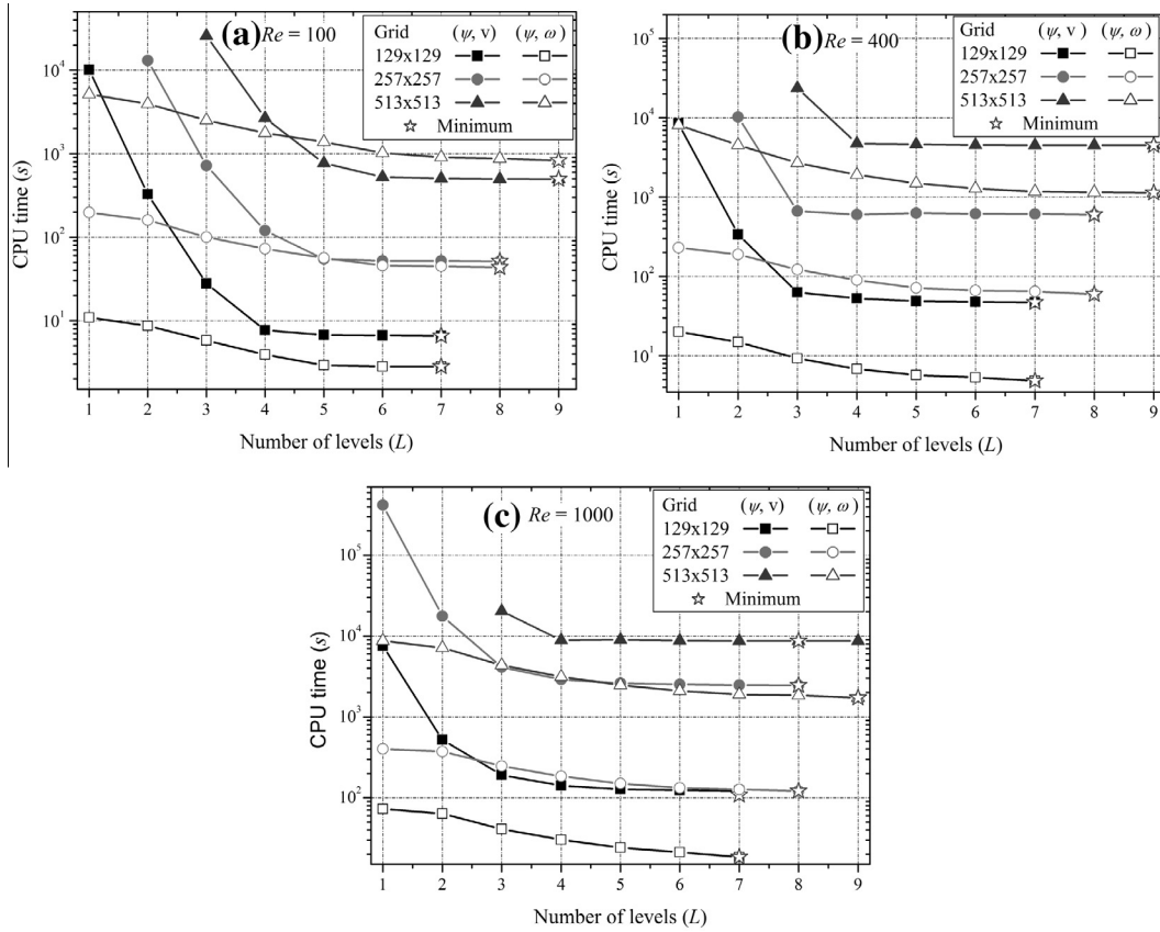
Fig. 6. Effect of number of levels on the CPU time for the Navier-Stokes equations.
