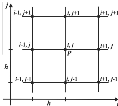
Fig. 1. Computational stencil.
