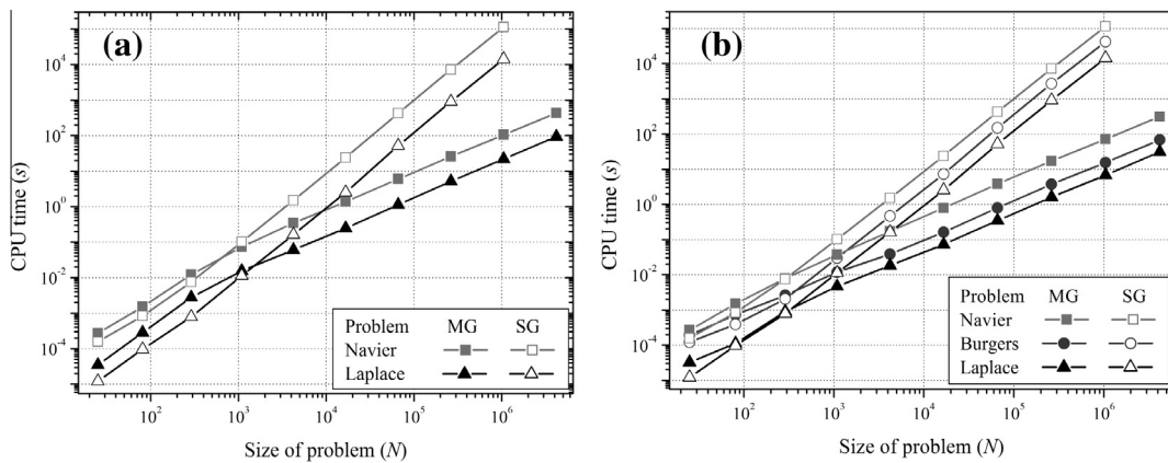
Fig. 7. Effect of problem size on CPU time for Laplace, Navier and Burgers equations: (a) CS scheme; (b) FAS scheme.
