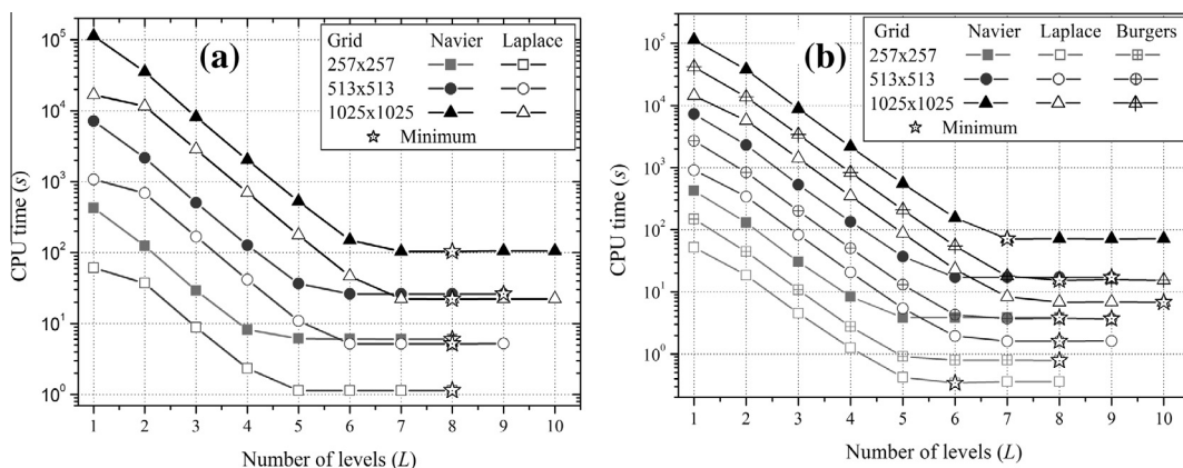
Fig. 5. Effect of number of levels ( L ) on the CPU time: (a) CS scheme; (b) FAS scheme.
