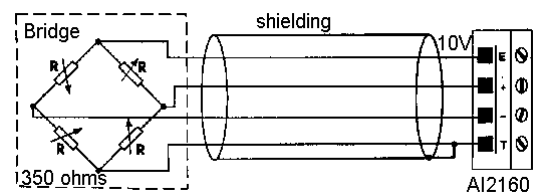
Fig. 5. Connecting the load cell to the Conditioner
