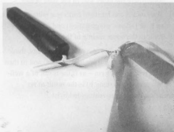
Figure 6-4i Streamer attachment to shock cord.
