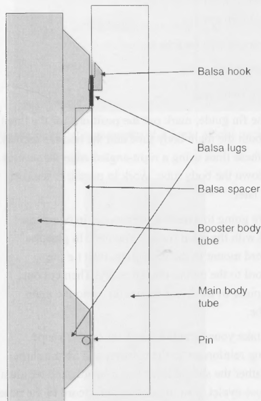
Figure 5-13 Parallel rocket mounting hardware.
