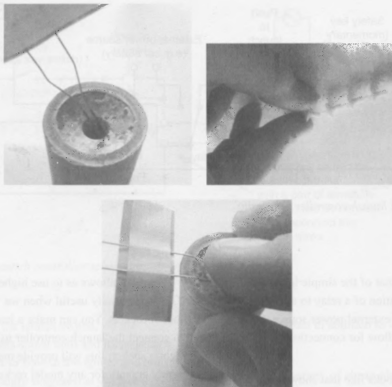
Figure 7-8 1) Insert the igniter into the throat of the model rocket motor. 2) Now take one of the small plastic plugs supplied with your motor. 3) Push the plug into the throat as far as it will go and you are ready to rock(et) and roll!
