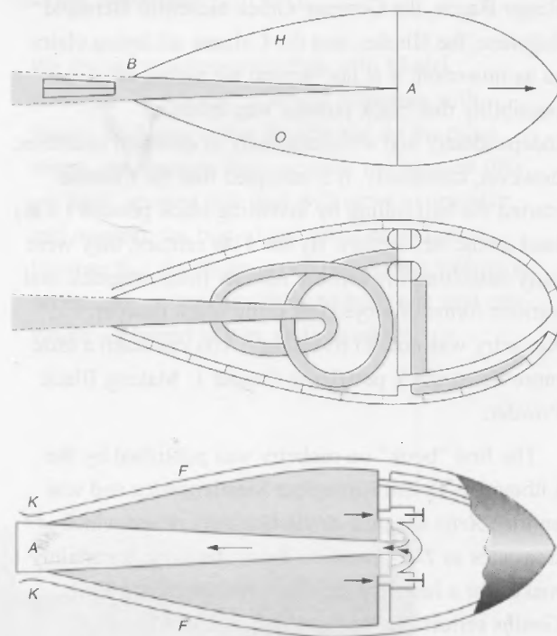
Figure 1-4 Some of Tsiolkovsky's rocket designs. Image courtesy NASA.
