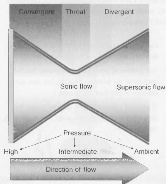
Figure 2-3 The de Laval nozzle.
