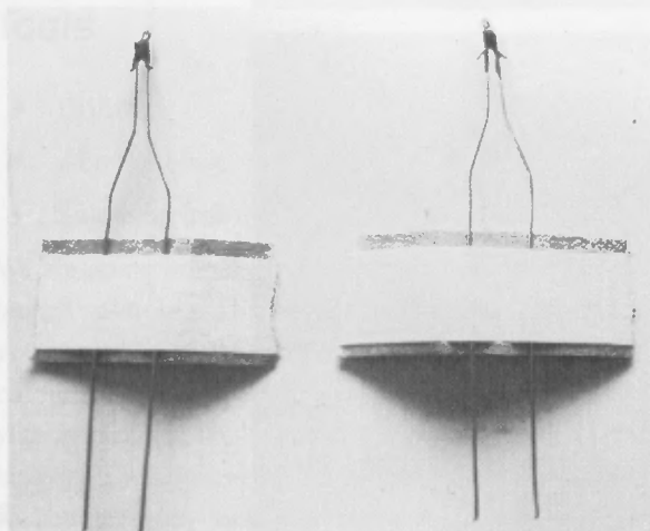
Figure 7-1. Rocket igniter construction.
