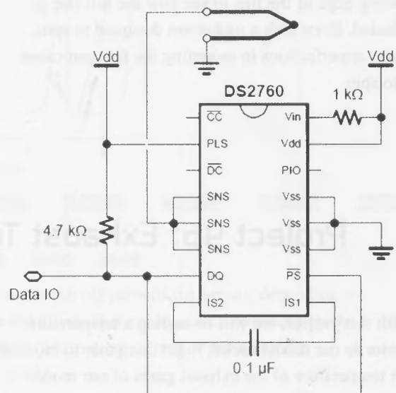
Figure 12-24 Thermocouple schematic.
