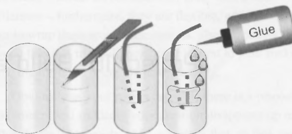
Figure 6-8 Through-tube method of mounting shock cords.
