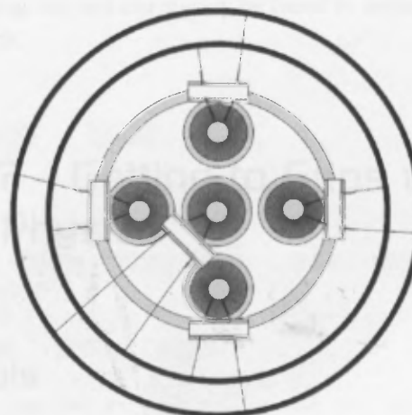
Figure 7-48 Wiring igniters for cluster motors.
