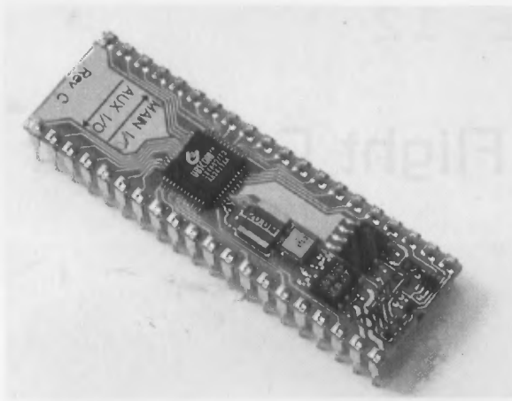
Figure 12-2 The BS2p40 chip.
