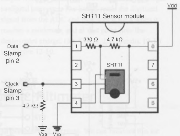
Figure 12-14 SHT 11 connection diagram.
