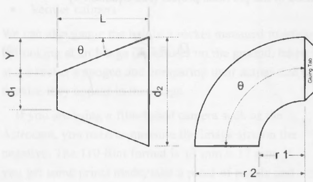
Figure 8-5 Critical transition dimensions.
