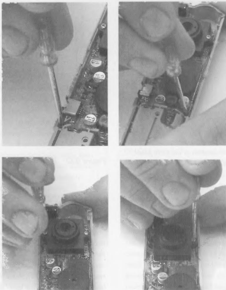
Figure 9-7 Removing the four screws inside the case.
