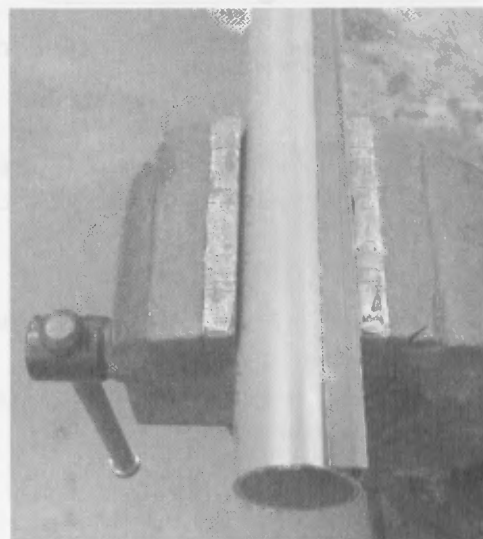
Figure 5-6 Clamping the body tube in order to mark it for fins or a launch lug.
