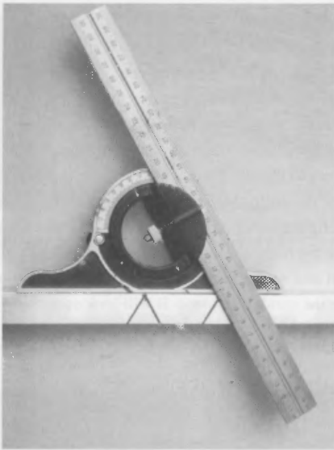
Figure 7-21 Marking out the aluminum angle.
