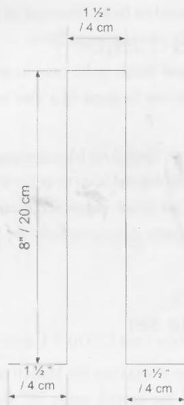
Figure 7-37 Bending diagram for metal bar.
