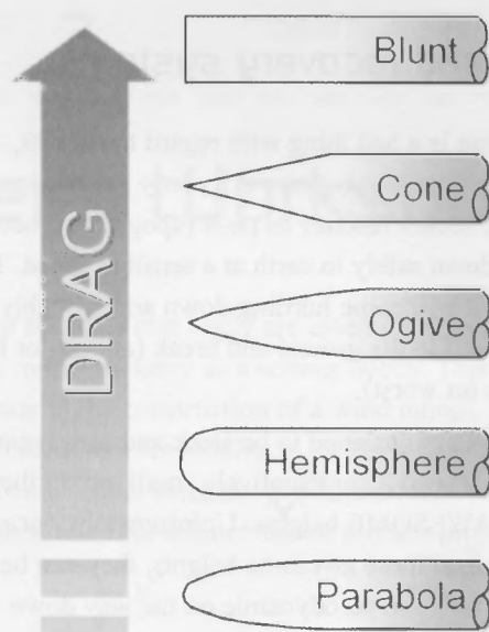
Figure 2-10 How nose cone profile affects drag.
