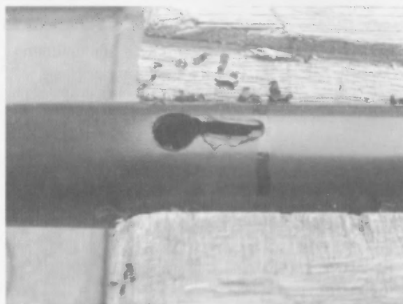
Figure 7-18 Hole and slot cut into electrical conduit.
