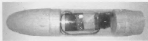
Figure 9-15 Model rocket camera installed prior to painting.
