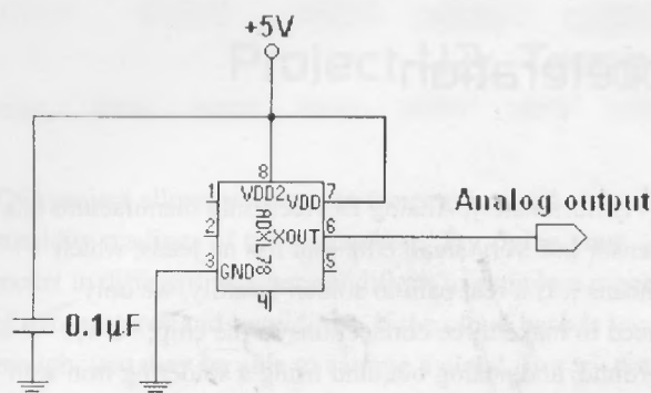
Figure 12-15 ADXL 78 connection diagram.
