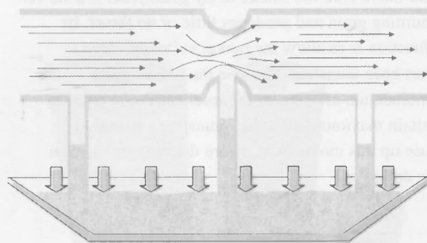
Figure 2-4 The Bernoulli effect.
