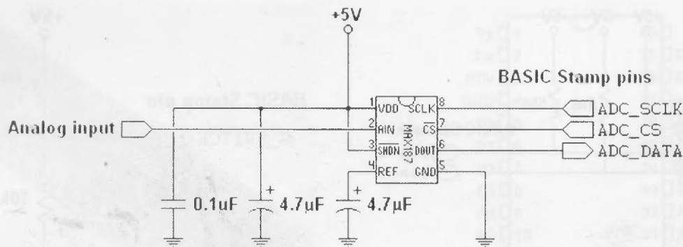
Figure 12-7 MAX 187 connection diagram.
