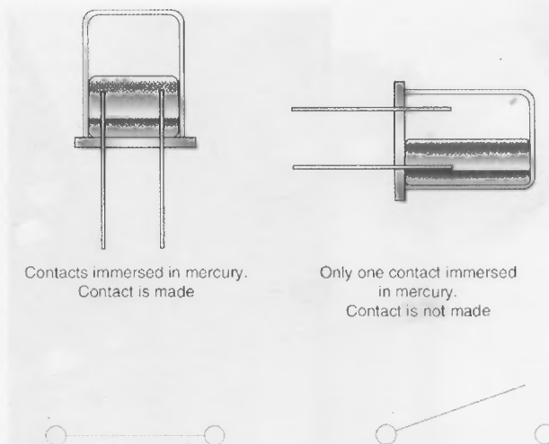
Figure 9-12 Tilt switch operation.
