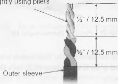
Figure 12-23 How to prepare the thermocouple.
