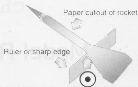
Figure 4-4 Finding the approximate center of pressure using a paper cutout.
