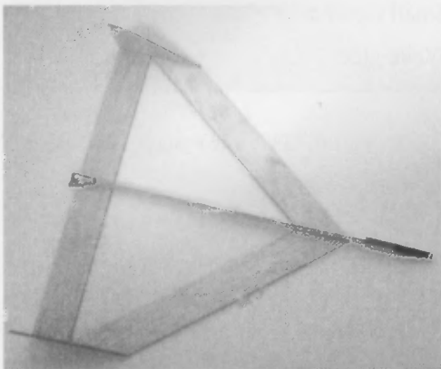
Figure 5-14 Finished balsa model.
