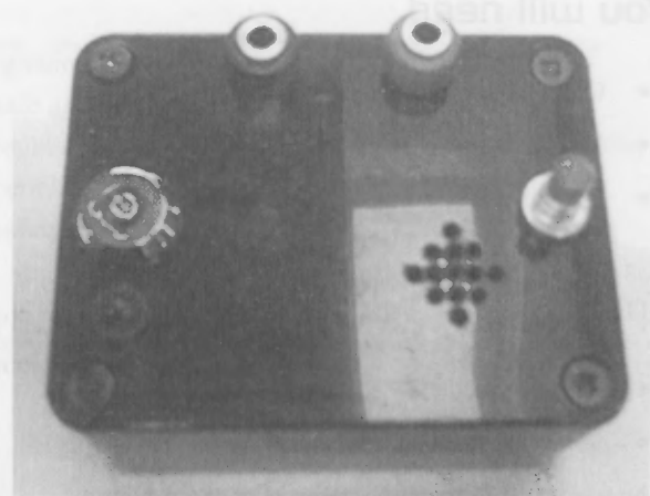
Figure 7-4 Assembled simple launch controller.
