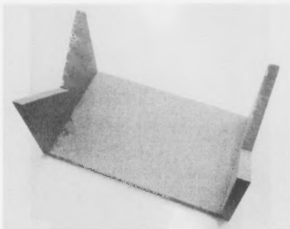
Figure 3-2 Model Rocket Support Jig.
