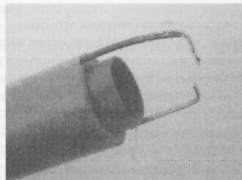
Figure 12-25 Mounting the thermocouple.
