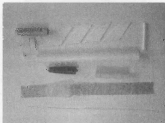
Figure 5-11i Components of a basic model rocket.
