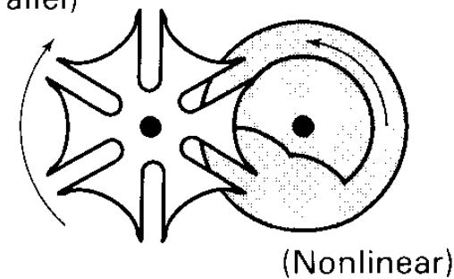
Geneva Wheel: (Parallel)
