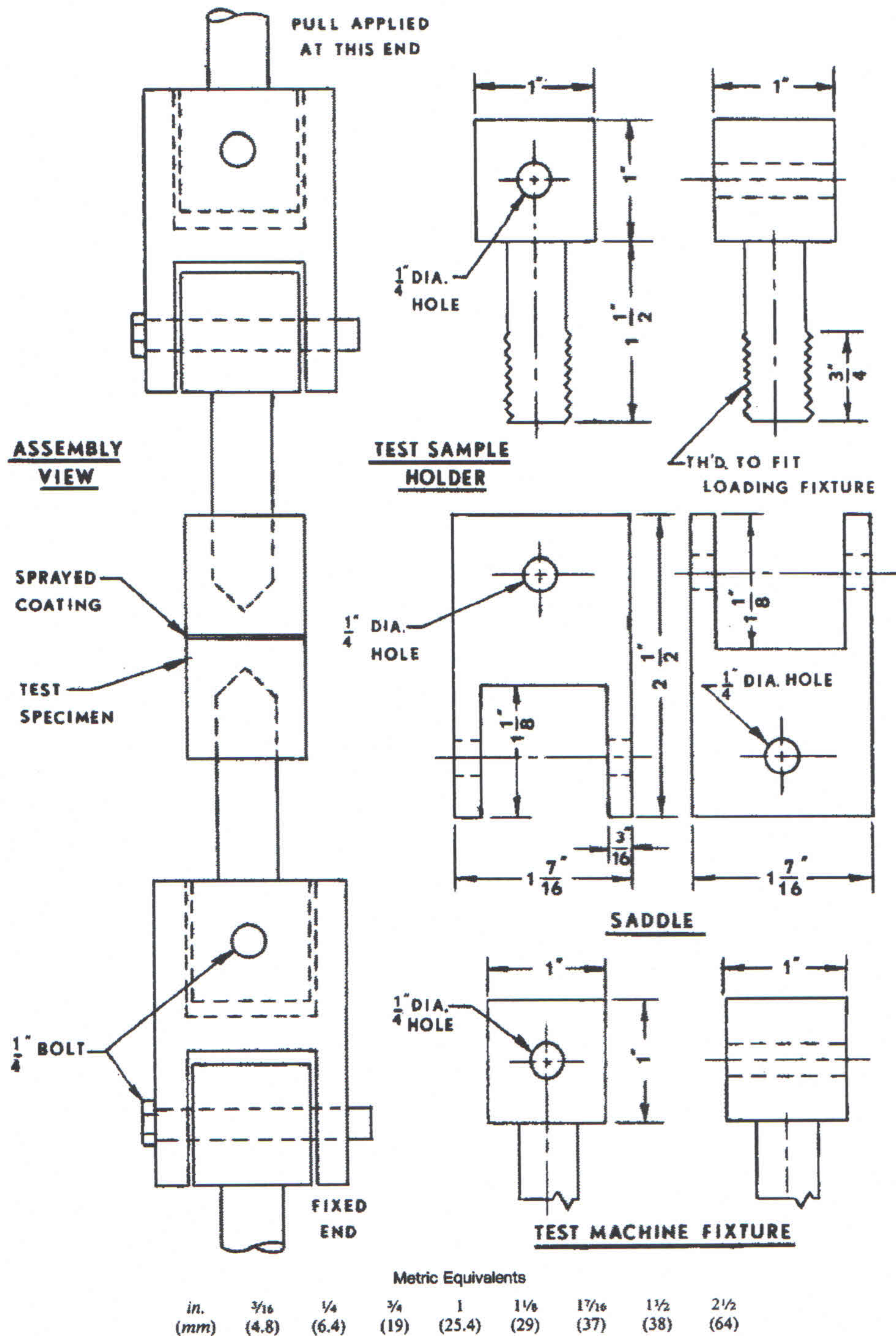
FIG. 1 Self-Aligning Device
