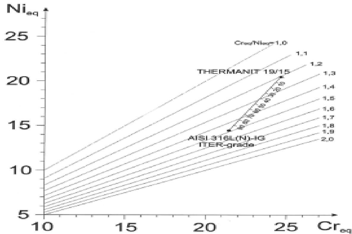
Figure 17. Cr eq and Ni eq values of parent and filler material placed in Hammar & Svensson diagram.
