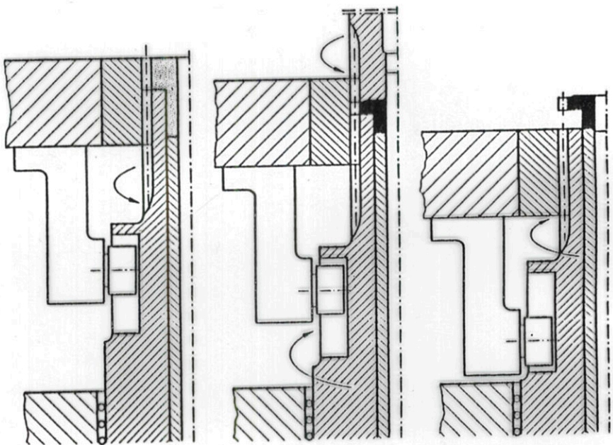
(above and opposite) Fabrication of critical geometries by axial pressing (for explanation see text) (Beiss)
