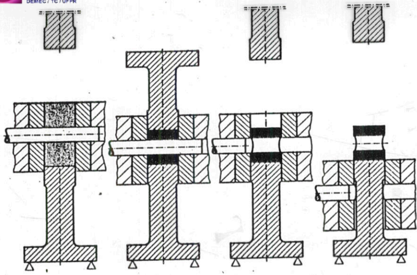
pressing of cross hole compact
