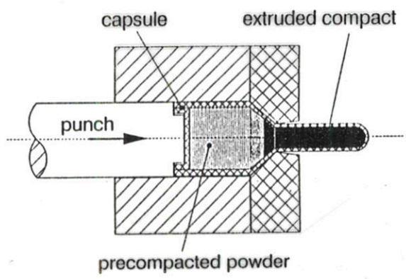
Hot powder extrusion of canned precompact powder
