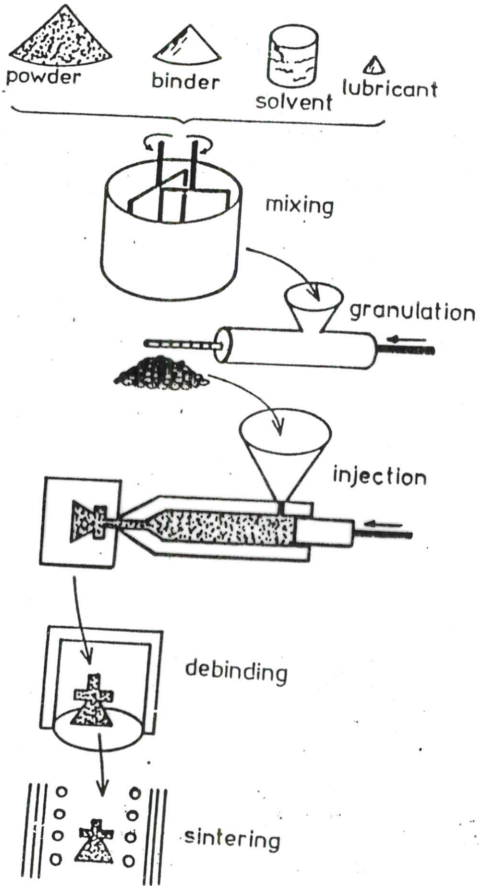
Figure 1. A schematic diagram of the processing steps and equipment involved in powder injection molding.
