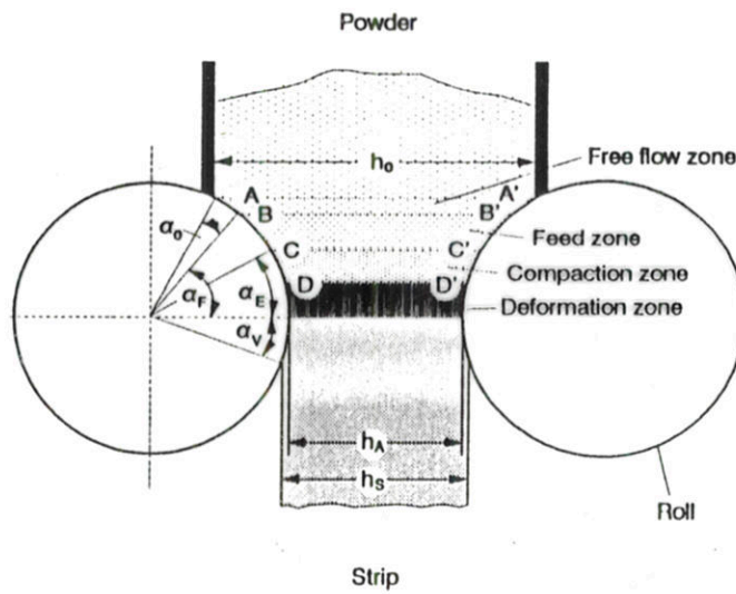
Powder/roll contact area in powder rolling (refer to text)
