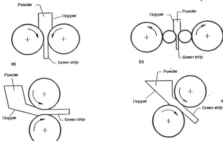
Powder/roll contact area in powder rolling (refer to text)
