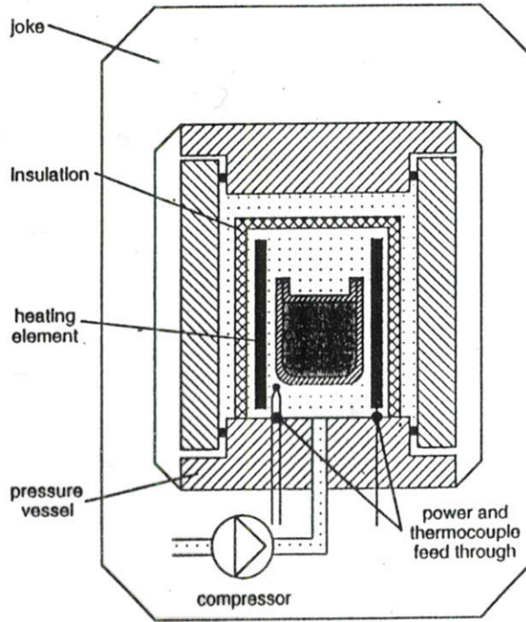
HIP components (schematic)
