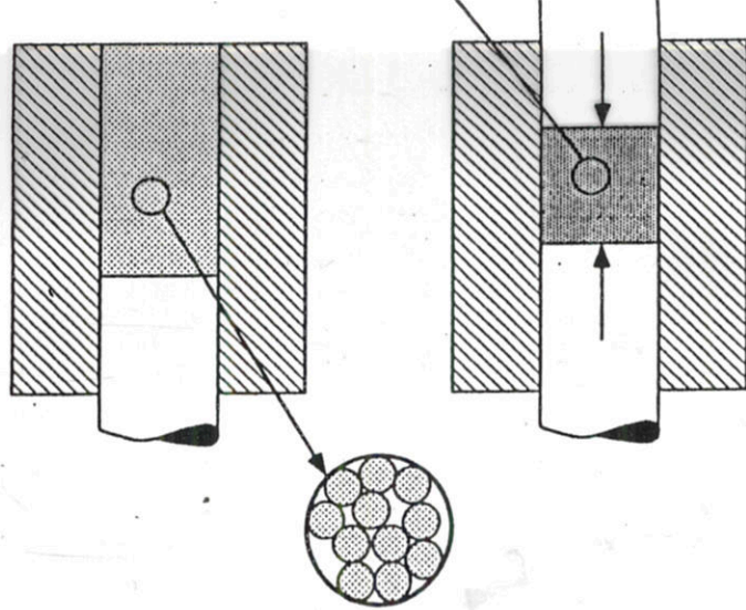
Densification during compaction by changes in particle arrangement and shape
