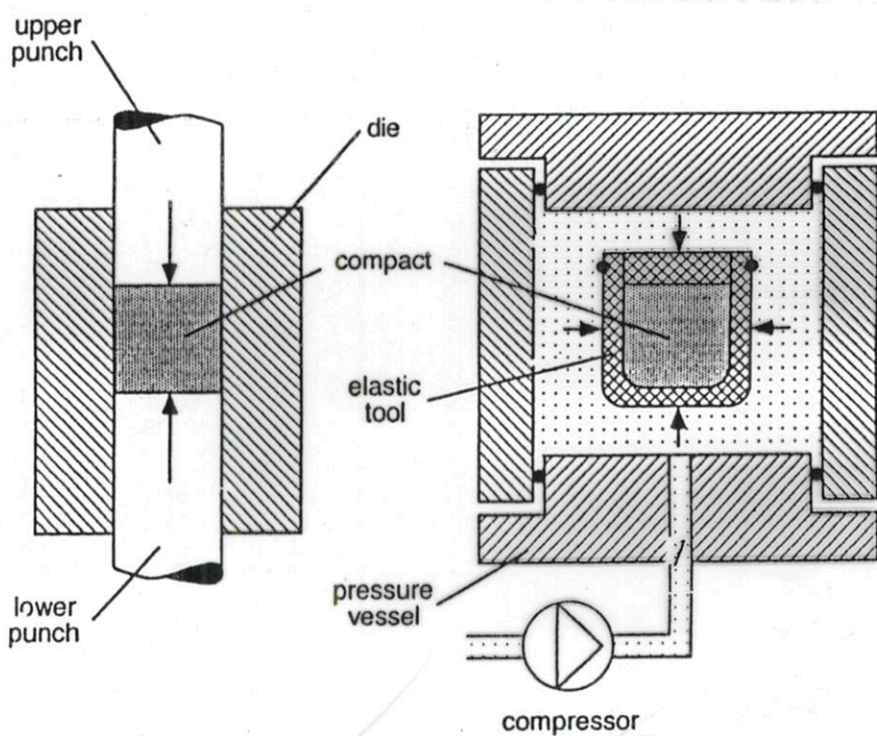
Cold pressing principles (left: axial- resp. die-pressing; right: isostatic pressing)
