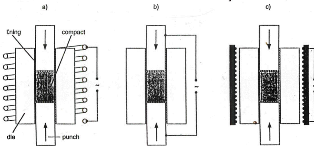
Tooling for axial hot pressing. a) induction heating; b) direct current heating; c) convection/radiation heating
