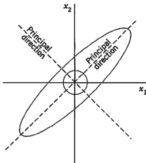
Fig. 158. Undeformed and deformed membrane in Example
