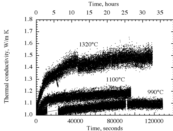
Figure 6 The overall thermal conductivity change kinetics of the \text{ZrO}_2\text{-Y}_2\text{O}_3 thermal barrier coating determined by the real time laser heat flux testing.
