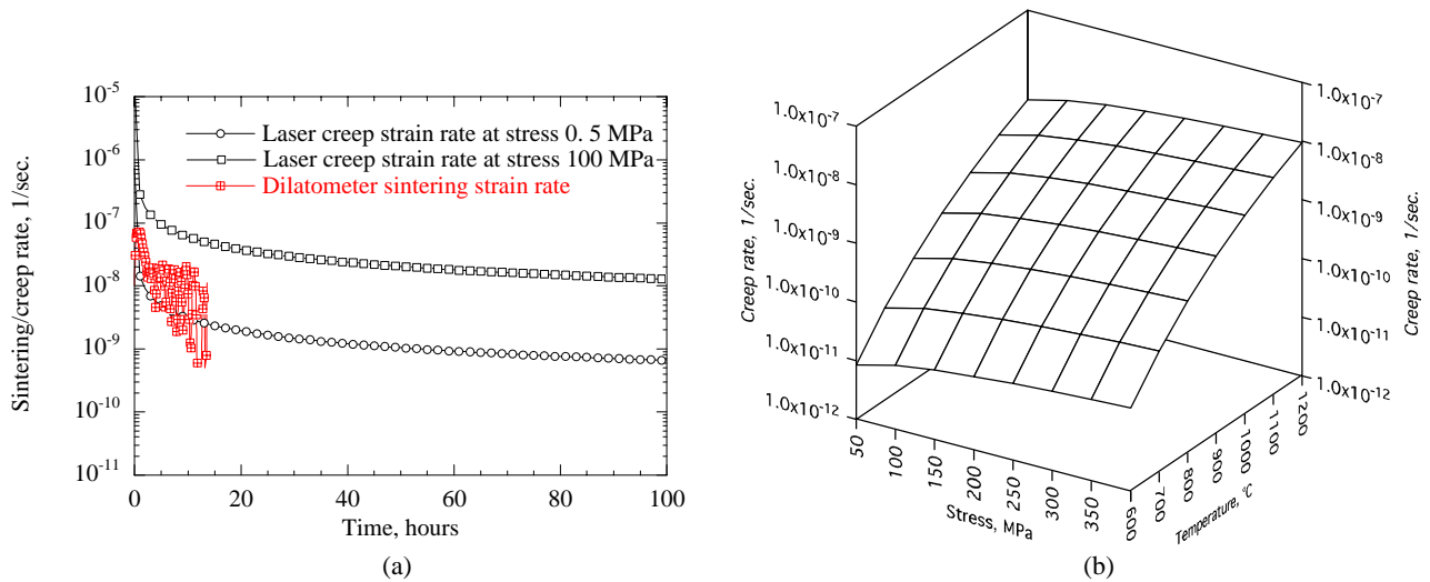
Figure 4 The sintering and creep characteristics of a plasma-sprayed ZrO_2 - Y_2O_3 coating material. (a) Sintering and creep rates as a function of time determined by the dilatometer sintering technique and the laser sintering/creep technique. The coating low stress (0.5 MPa) creep rates obtained from the laser creep test are in good agreement with the coating sintering rates obtained from the dilatometer test. (b) Stress- and temperature-dependence of the creep rate for a ZrO_2 -8% Y_2O_3 thermal barrier coating (at 500 hours).
