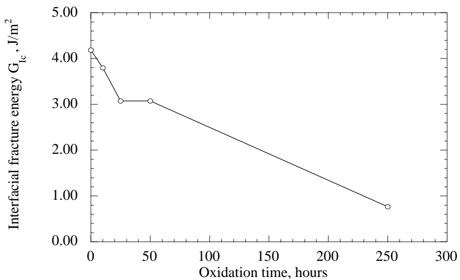
Figure 12 Ceramic/bond coat interfacial fracture energy as a function of oxidation time for a ZrO_2 -8% Y_2O_3 /Ni-36Cr-5Al-Y bond coat/CMSX-4 substrate system oxidized at 1100°C. (Mechanical properties used for the critical energy release rate calculation: E_c = 30GPa , E_m = 190GPa , \nu_c = 0.25 , \nu_m = 0.27 ).
