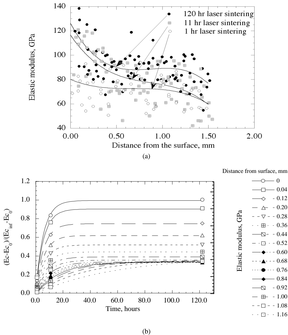
Figure 8 Elastic modulus evolution in a ZrO_2 - Y_2O_3 thermal barrier coating under laser heat flux sintering and creep conditions. (a) The elastic modulus distributions in the ZrO_2 - Y_2O_3 thermal barrier coating as a function of laser sintering time. (b) The experimentally determined modulus change kinetics across the coating system.
