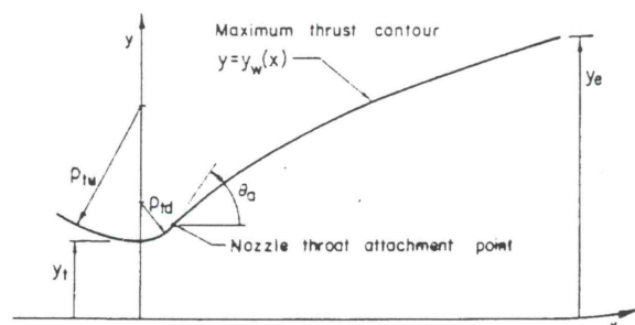
Fig. 1 Nozzle flowfield model.
