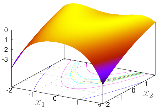
Figure 4: Rosenbrock function.
