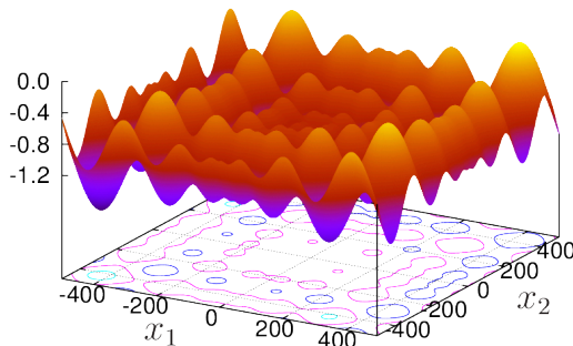
Figure 6: Schwefel 2.26 function.
