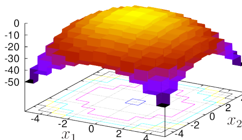
Figure 3: Step function.
