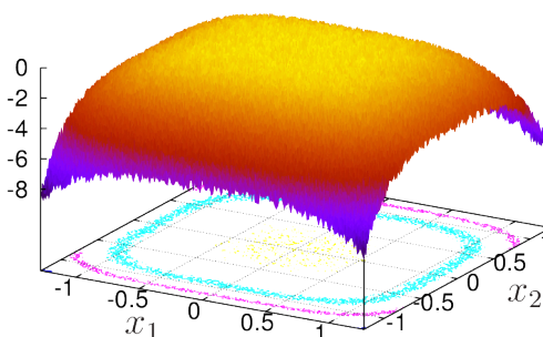
Figure 5: Noisy Quartic function.
